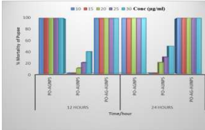
Figure 6: Percentage mortality (%) of Pupae in 12 and 24 hours at different concentrations of synthesized AgNPs, AuNPs, and Ag-AuNPs using Pleurotus ostreatus (PO)
