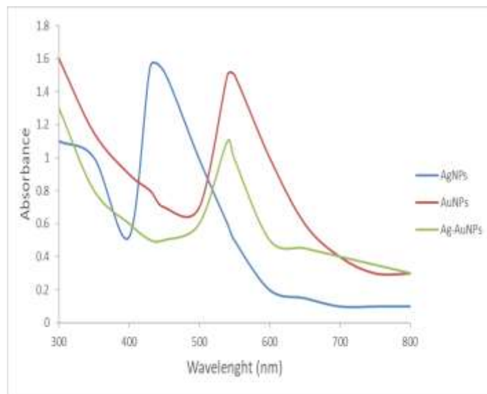
Figure 1: UV-vis spectroscopy of Pleurotus ostreatus Biosynthesized AgNPs, AuNPs, Ag-AuNPs
