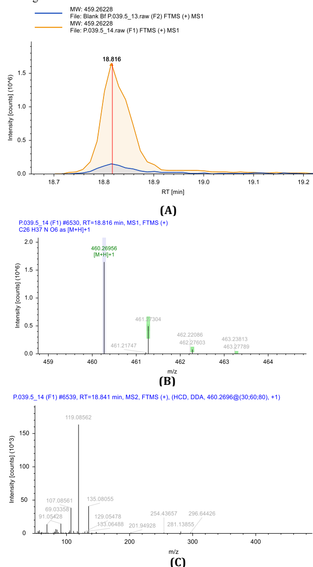
Figure 6: LC-HRMS/MS spectrum of B. safensis crude extract corresponding to militarinone A. (A - B) The extracted mass spectrum of militarinone A at [M+H]^+ at m/z 460.26956 with RT 18.816 min, (C) The MS2 spectrum of militarinone A with its in-source fragments
