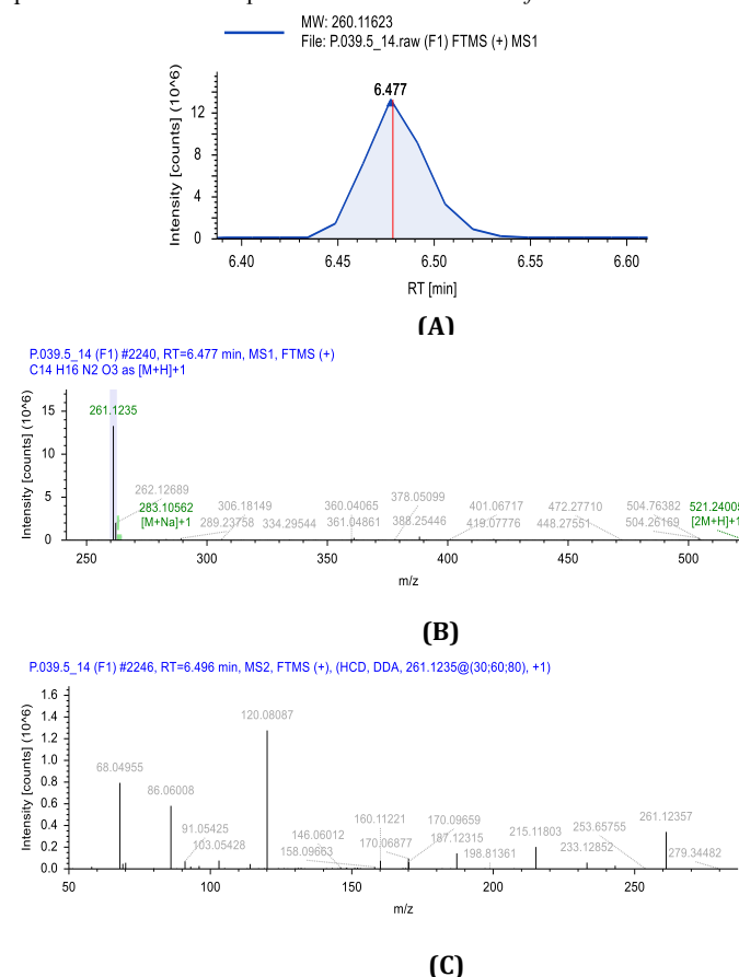
Figure 7: LC-HRMS/MS spectrum of B. safensis crude extract corresponding to maculosin. (A - B) The extracted mass spectrum of maculosin at [M+H]^+ at m/z 261.1235 with RT 6.477 min, (C) The MS2 spectrum of maculosin with its in-source fragments
