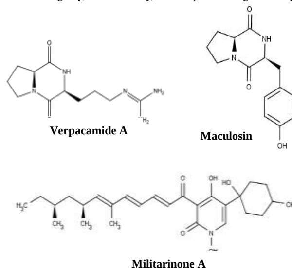
Figure 5: Putative structure of anticancer compounds namely verpacamide A, maculosin, and militarinone A found in B. safensis P.039.5 based on the mass spectra. These compounds exhibited potent binding affinities against ER- \alpha , HER2, EGFR, CDK2, and topoisomerase II \alpha .
