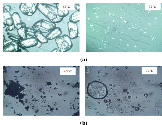
Figure 2: HSM analysis of thermal behavior and morphology of pure ibuprofen (IBU) and ibuprofen-nicotinamide cocrystals (IBU-NICO)
