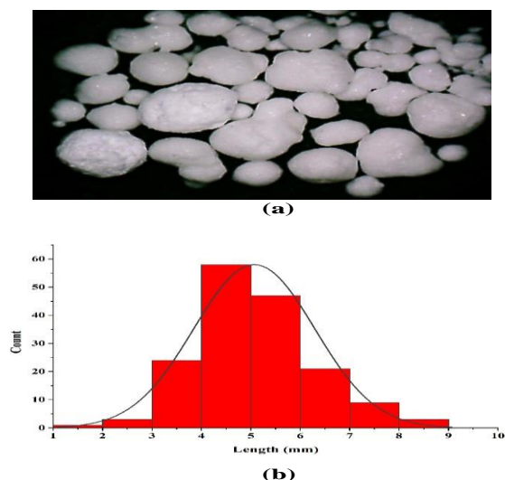
Figure 6: Morphology (a) and particle size distribution (b) of ibuprofen-nicotinamide cocrystals produced by spherical agglomeration-based spherical cocrystallization (SA-CC)
