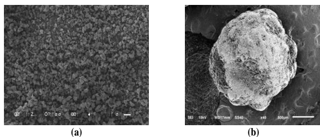
Figure 3: SEM analysis of ibuprofen crystals (a) and spherical ibuprofen-nicotinamide cocrystal (b)
