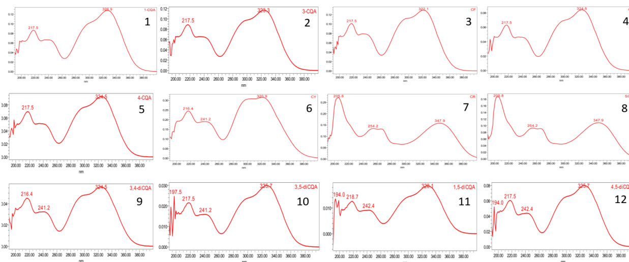
Figure 1. UV spectra of 12 phenolic compounds in artichoke leaf extract
