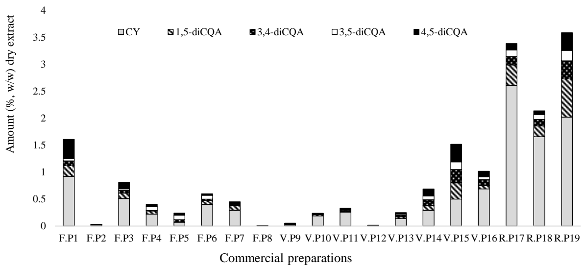
Figure 3: Amounts of di-CQAs of commercial artichoke supplements
