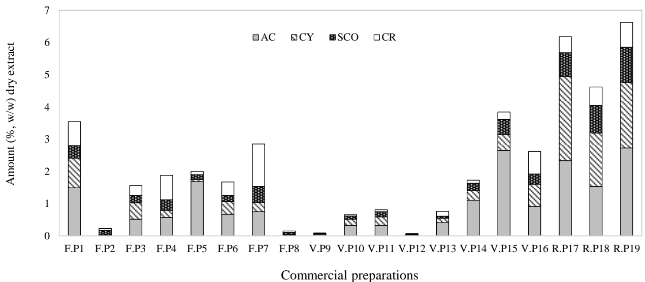
Figure 4: Amounts of major phenolic compounds of commercial artichoke supplements
