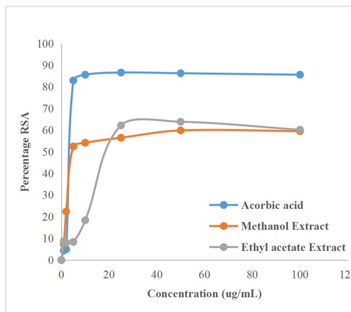
Figure 1: DPPH Radical Scavenging Activity of Extracts of Stachytarpheta jamaicensis leaves.
